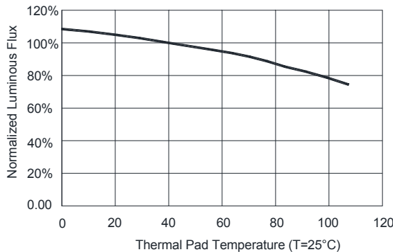
Thermal Pad Temperature vs. Relative Light Output
