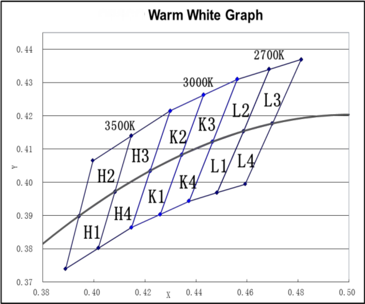
ANSI Warm White Color bin structures
